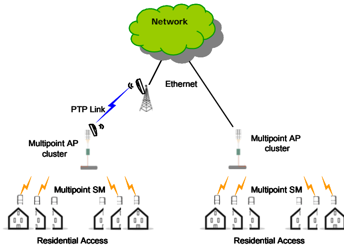
Figure 3: Motorola Wireless Networks Used for Residential Access
